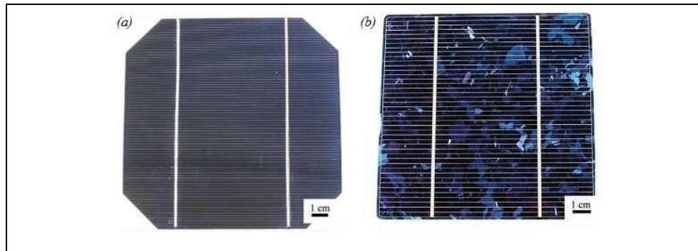
FIG 3. PHOTOGRAPHS OF (A) CRYSTALLINE, AND (B) MULTI-CRYSTALLINE SI SOLAR CELLS
